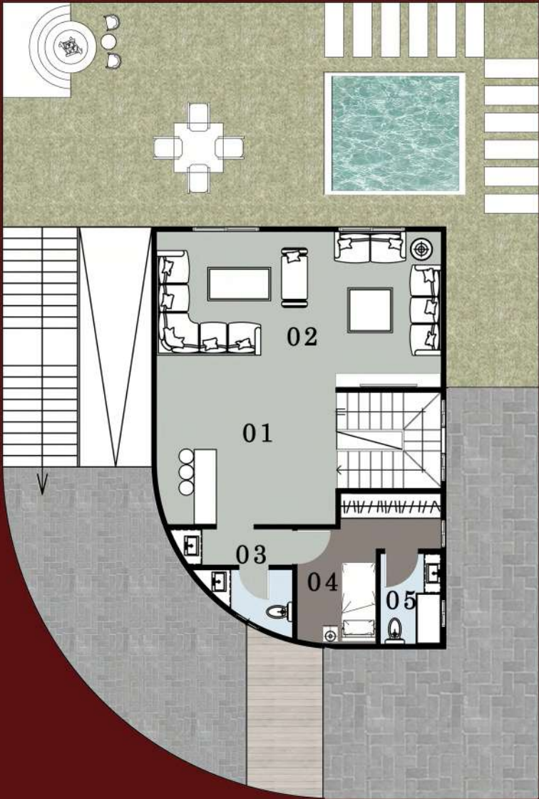
Walk out Floor Area: 131 m 2
