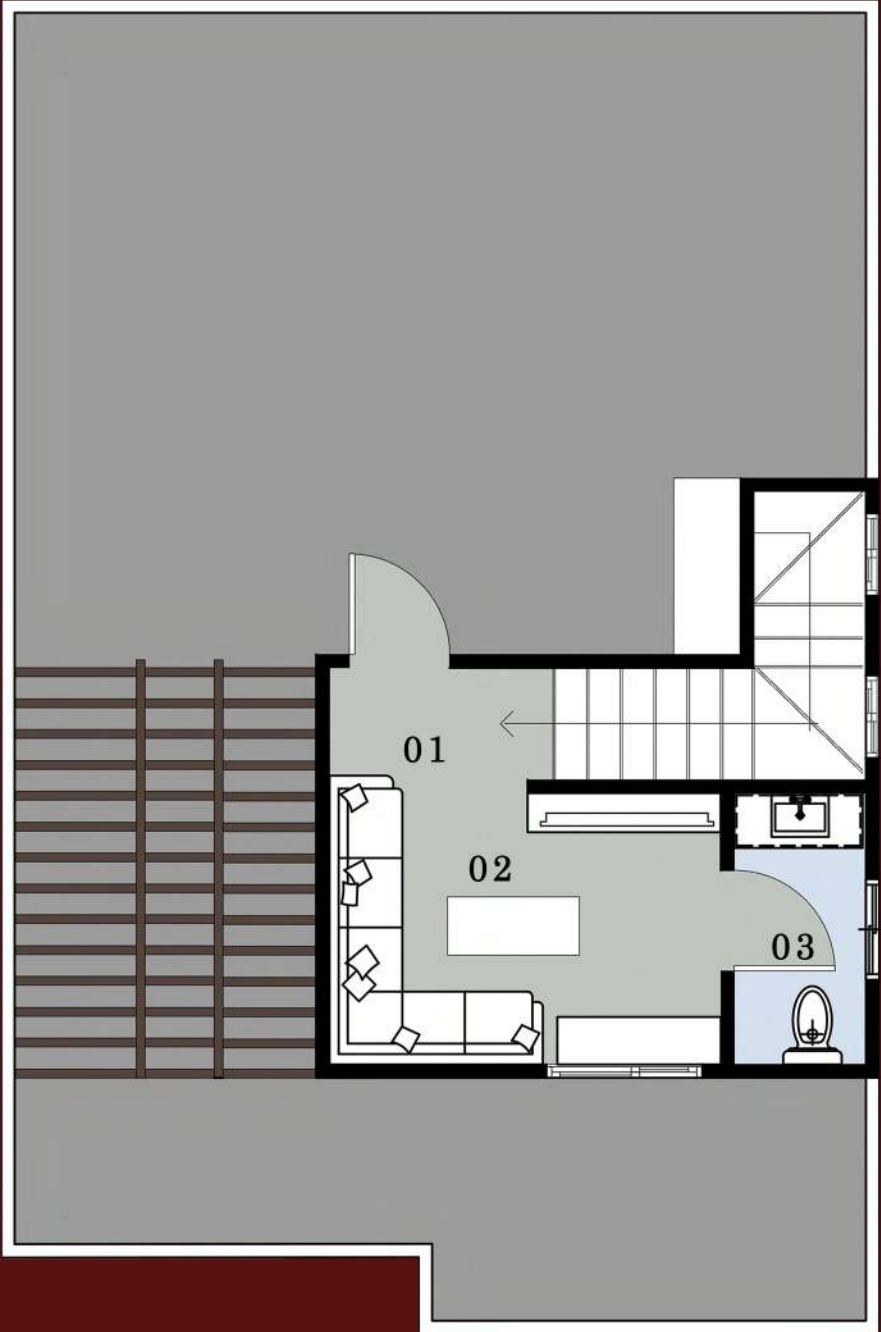
Roof Floor Area: 22 m2
